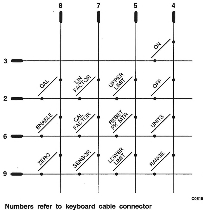
Fig. 1-2 Keyboard connections
